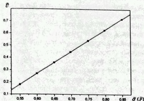
Fig 2. The regularity of the resulting average amplitude of the AE signal from the value of contact stress expressed in relative values. Data processing was carried out by the modelling results, in accordance with (1)
