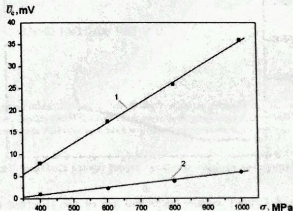
Fig 4. Regularity of the average amplitude of the AE signal (1) and the strain gauge transducer signal (2) from the unit value of contact pressure
