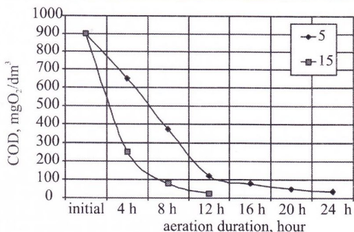
Fig. 1. Effect of active sludge concentration to reduce COD during aerobic wastewater treatment
