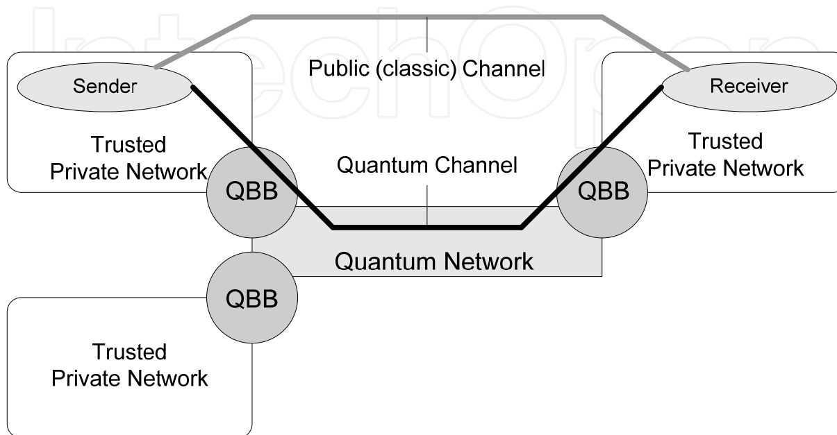
Fig. 6. Brief network architecture of SECOQC.
