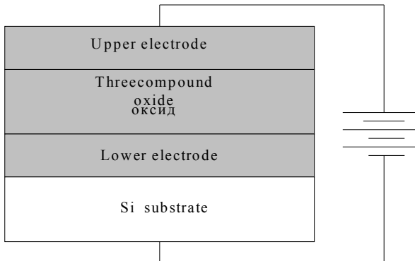
Fig. 6.8. MDM structure of the memristor
