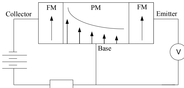
Fig. 7.11. The structure of the Jonson transistor
