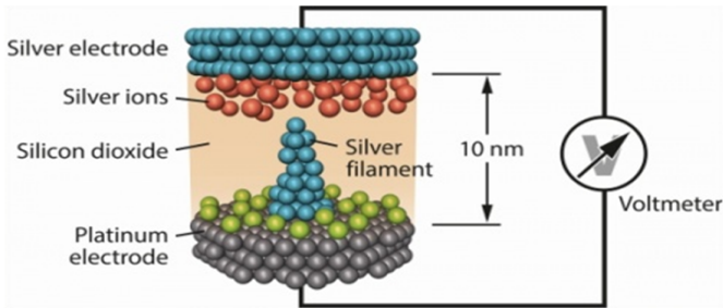
Fig. 5.13. Formation of the filament in the structure \text{Ag}/\text{SiO}_2/\text{Pt}
