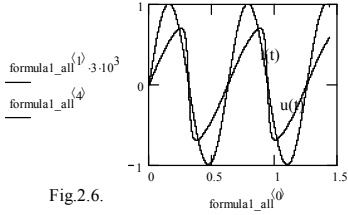
Fig. 2.6. The results of a memristor simulation
