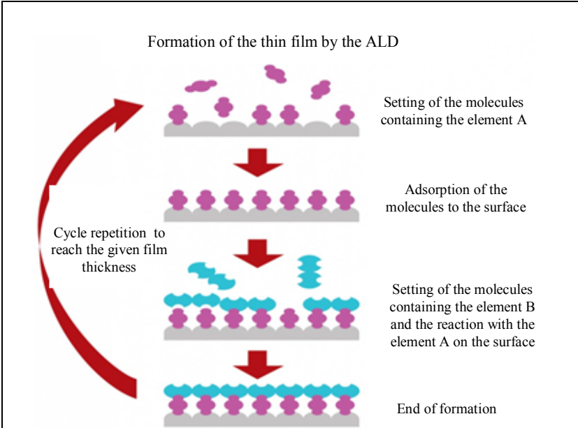
Fig. 6.15. Formation of the thin films by the ALD
