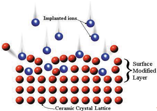
Fig. 6.9. The ion implantation process
