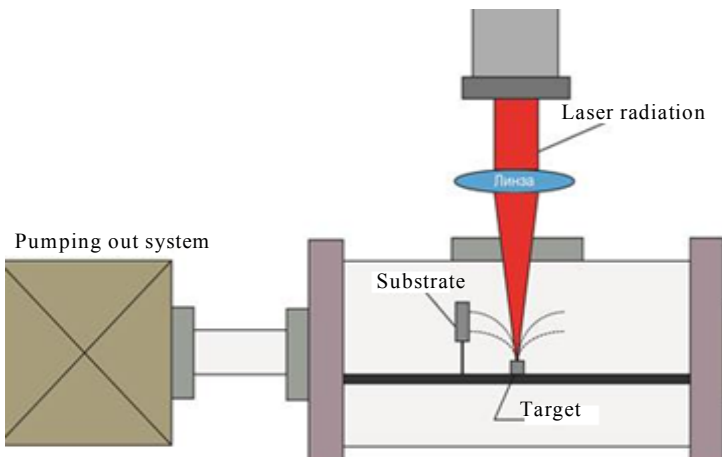
Fig. 6.17. Laser ablation of the target material
