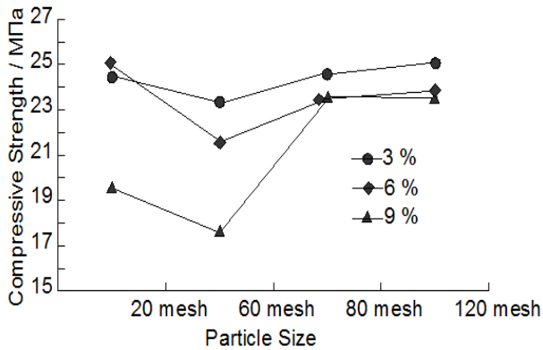
Fig. 1 The change of the particle size of 28d rubber concrete with the same amount rate
