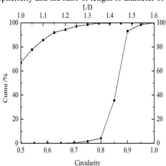
Fig. 1 Circularity and length to diameter ratio of rubber particles
