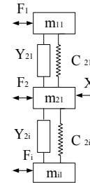
Fig. 2. A kinematic scheme for the propagation of low-frequency vibrations
