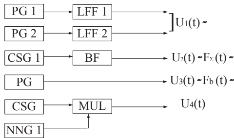
Fig. 5. A scheme of the model of force effects: PG – pulse generators; NNG – normal noise generator; CSG – code-sequence generator; LFF – low frequency filters; BF – bandpass filter; MUL – multiplier
