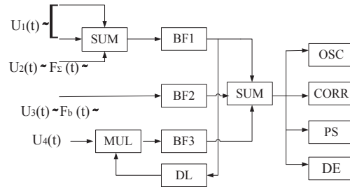
Fig. 6. A scheme of the model for the vibroacoustic effect propagation: SUM – signal summators; BF – bandpass filter; DL – delay line; OCS – oscilloscope; CORR – correlometer; PS – power spectrum analyzer; DE – signal probability density analyzer
